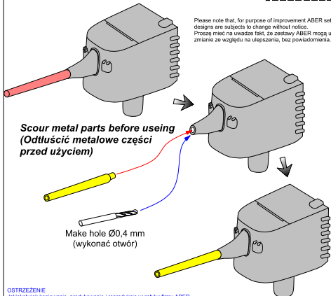
Main 140mm Gun
