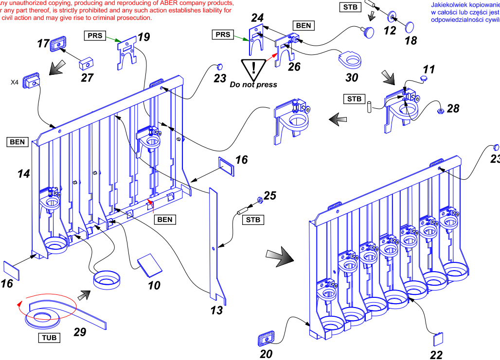
Left & right ammo box symmetrical assembled
