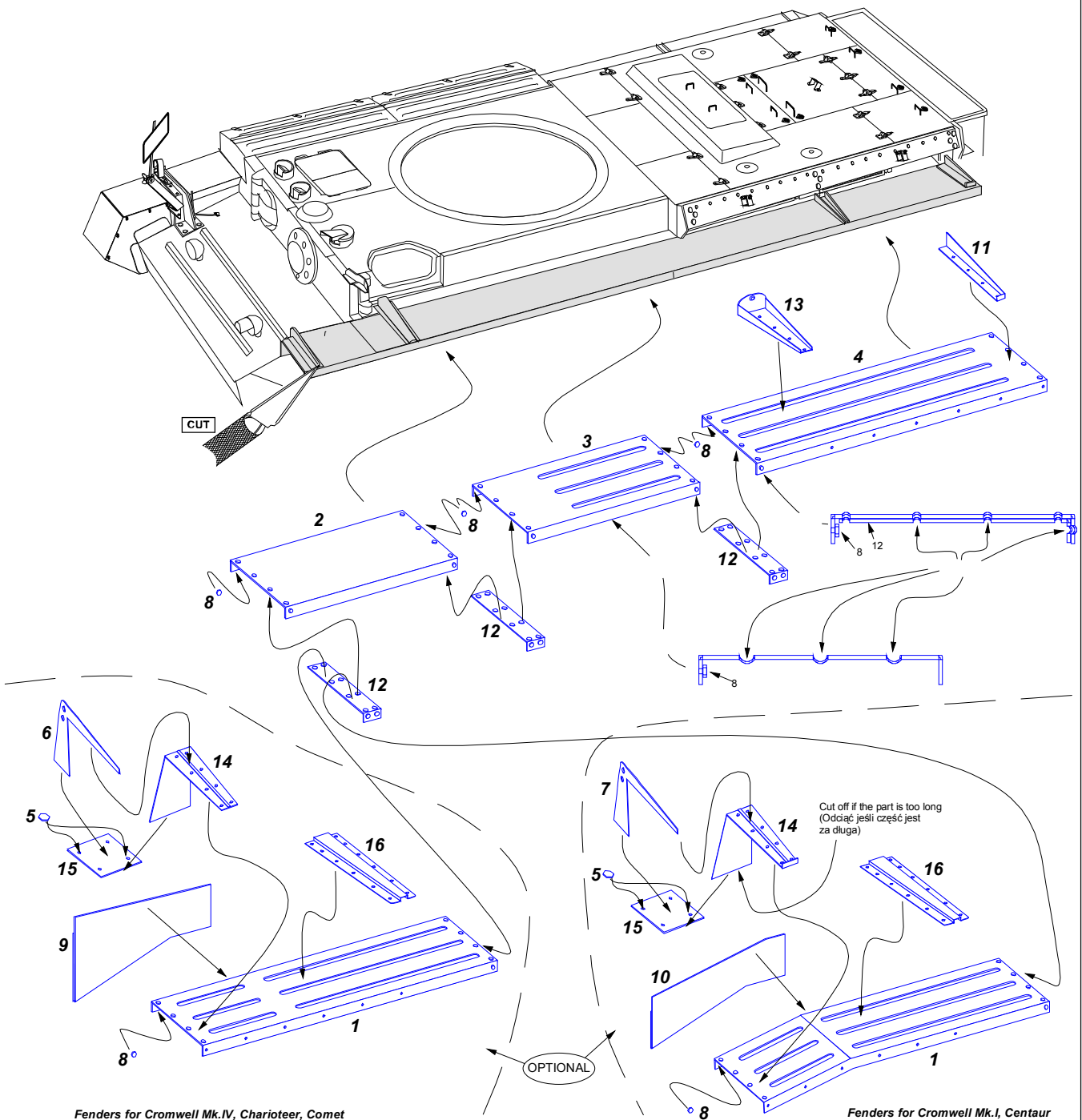
Fenders for Cromwell Mk.IV, Charioteer, Comet
