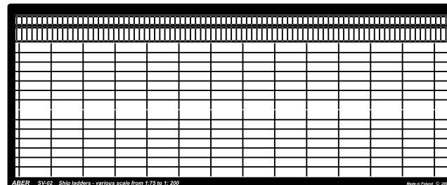
ABER SV-02 Ship ladders - various scale from 1:75 to 1:200
